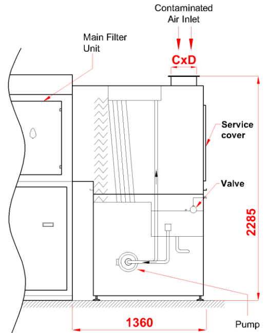
Water Pre-separator (With AC-163 filter unit)
